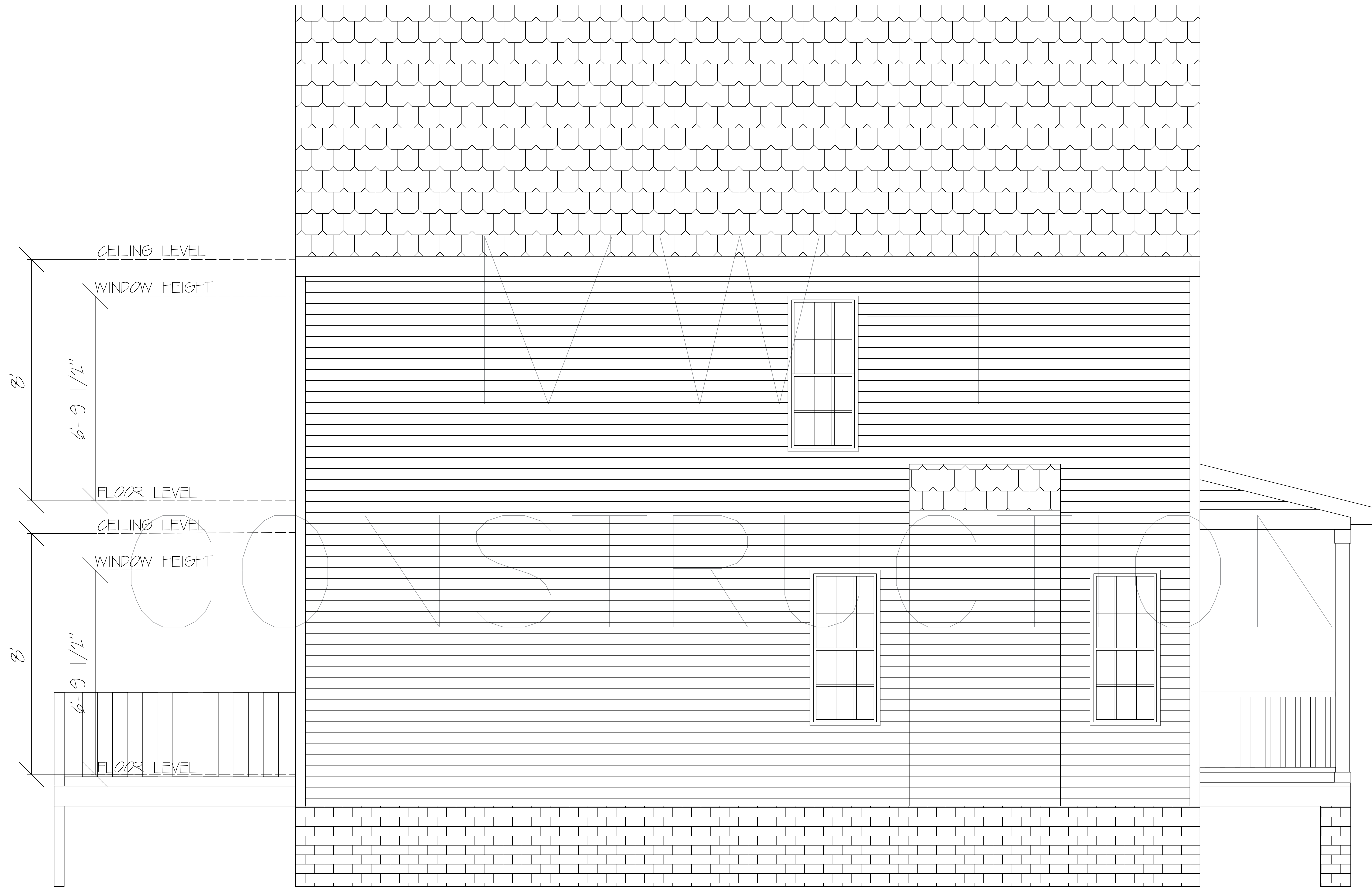
LEFT ELEVATION VIEW
